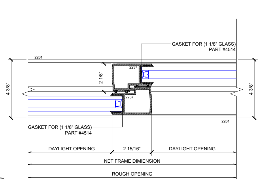
⑤ 90° CORNER DETAIL MAX SLIDING DOORS (OXXO) SCALE: 6"=1'-0"
