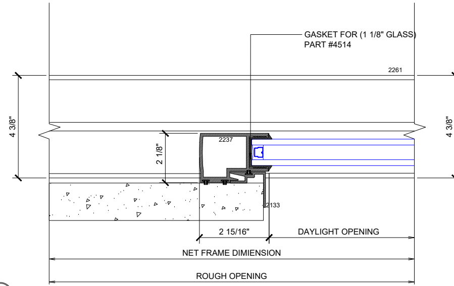
② VERTICAL MAX SLIDING DOORS (OXXO) SCALE: 6"=1'-0"
