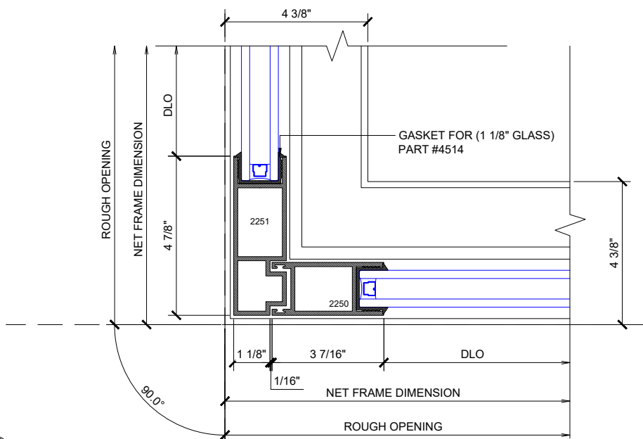
④ 90° CORNER DETAIL MAX SLIDING DOORS (OXXO) SCALE: 6"=1'-0"
