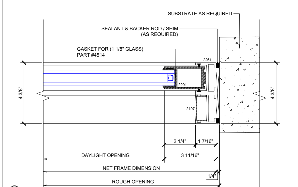
⑥ VERTICAL MAX SLIDING DOORS (OXXO) SCALE: 6"=1'-0"
